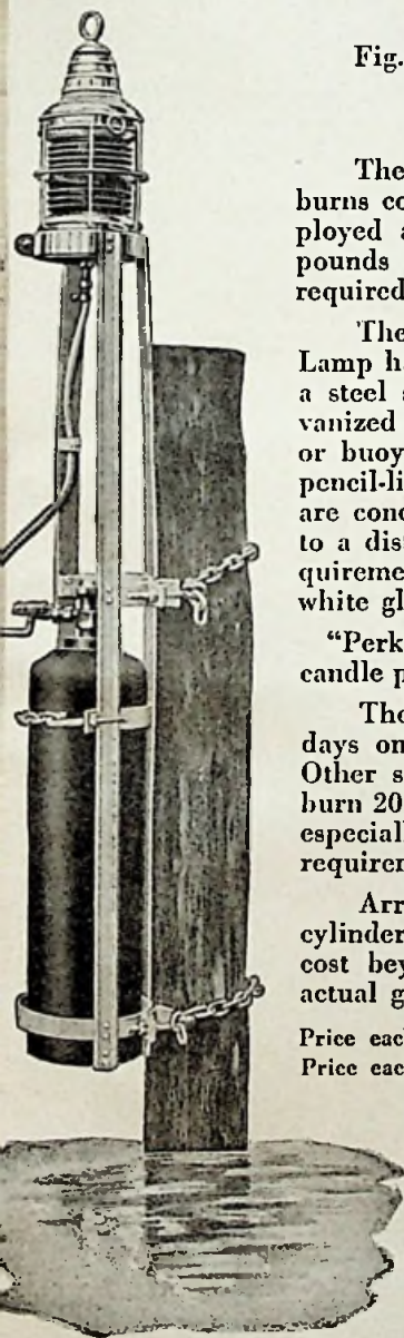
Fig. 109a Complete Beacon in Place on a Pile
